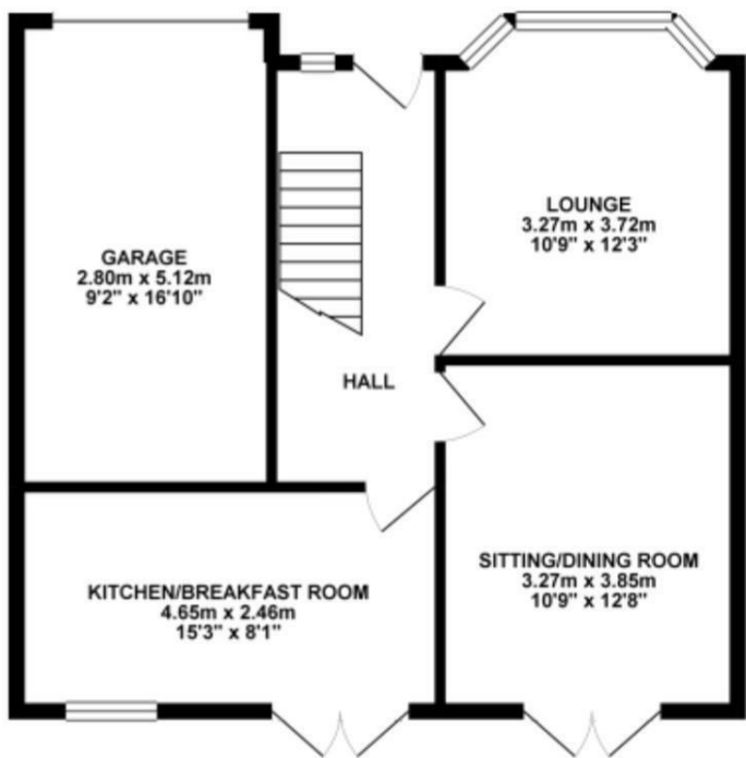
GROUND FLOOR 58.71 sq. m. ( 631.90 sq. ft. )
